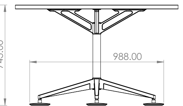
RIGHT-SIDE VIEW
