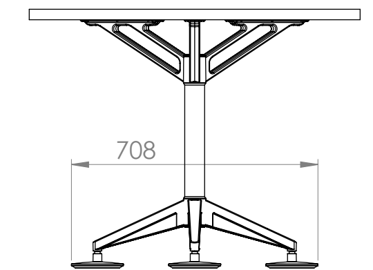
RIGHT-SIDE VIEW
