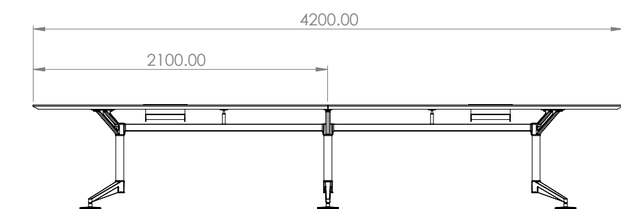
RIGHT-SIDE VIEW
