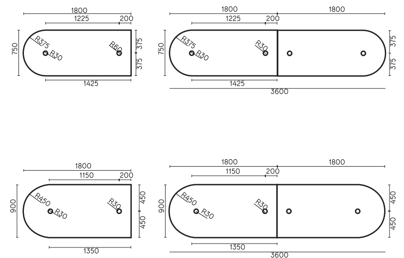
Twelve Student Boardroom Table Created with two 1800x750mm Teknik Tables
