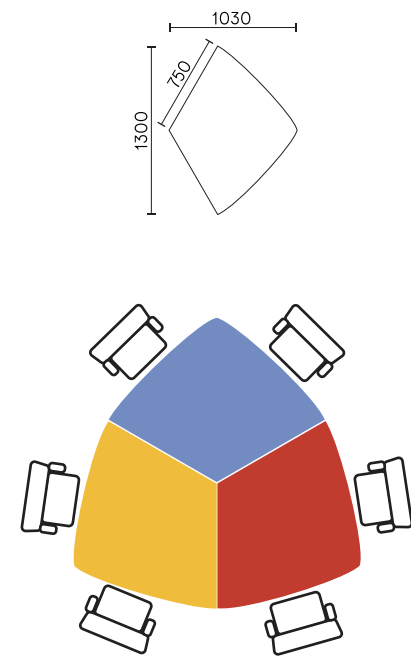
Six Student Large Stingray Configuration Created With Three 1300mm 1030mm Stingray Tables
